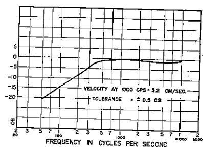
Fig. 12—Average calibration of 45 revolution-per-minute test record 12-5-31.
