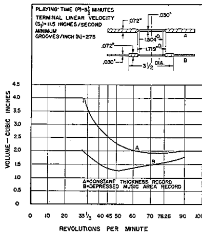
Fig. 10—Relation of record volume to rotational speed for (A) Constant thickness record, (B) depressed music area record with constant diameter label.
